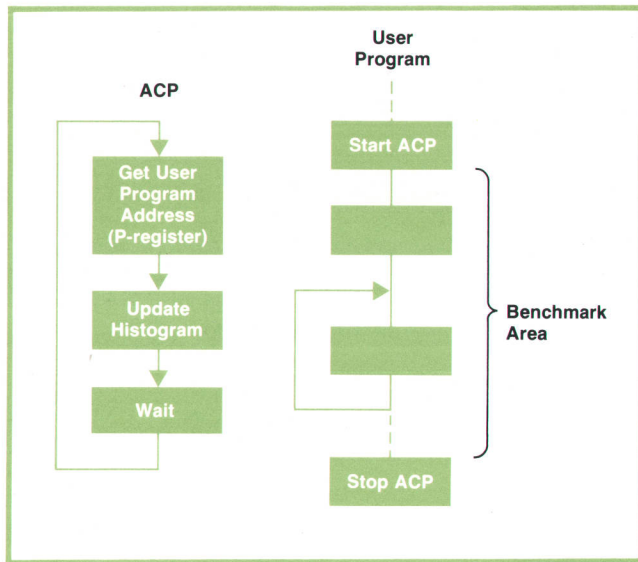
Fig. 4. The activity profile, a plot showing the percentage of time spent in each area of memory, is an excellent tool for timing analysis. Generating it requires that the program labeled ACP run at the same time as the user's program. Any computer's interrupt system provides this capability.
