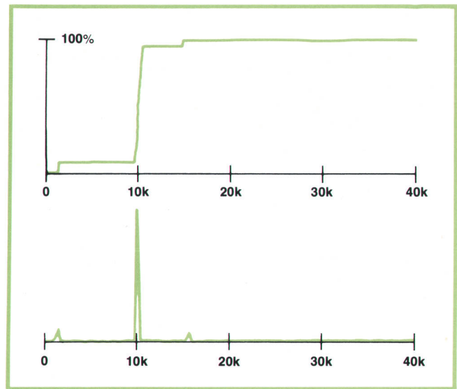
Fig. 10. Activity profile for a benchmark process used in the 5451A shows that 80% of the time is spent in subroutines near memory location 10000s.
