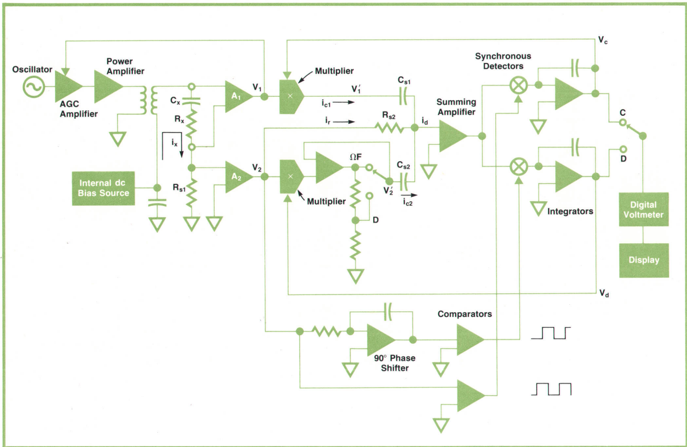
Fig. 3. Simplified circuit diagram of the 4282A Digital High-Capacitance Meter. The transformer makes it possible to apply dc bias to the unknown along with the ac test signal at 50, 60, 100, or 120 Hz.
