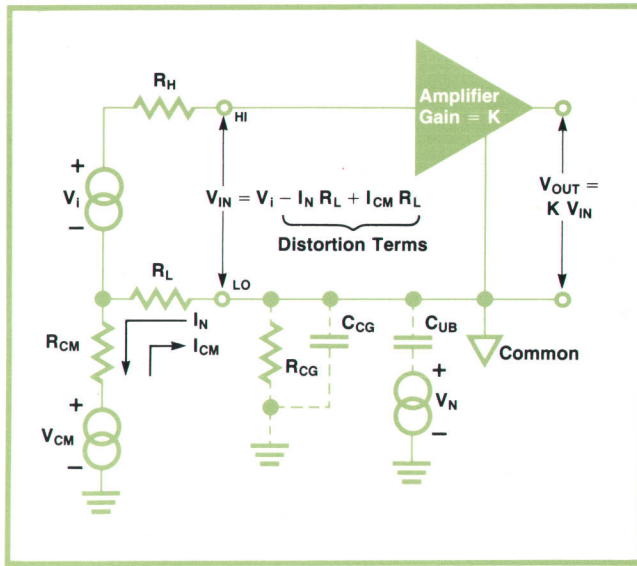
Fig. 5. Conventional input amplifiers have problems because of pump-out and common-mode currents flowing through the source resistance, R_L .
