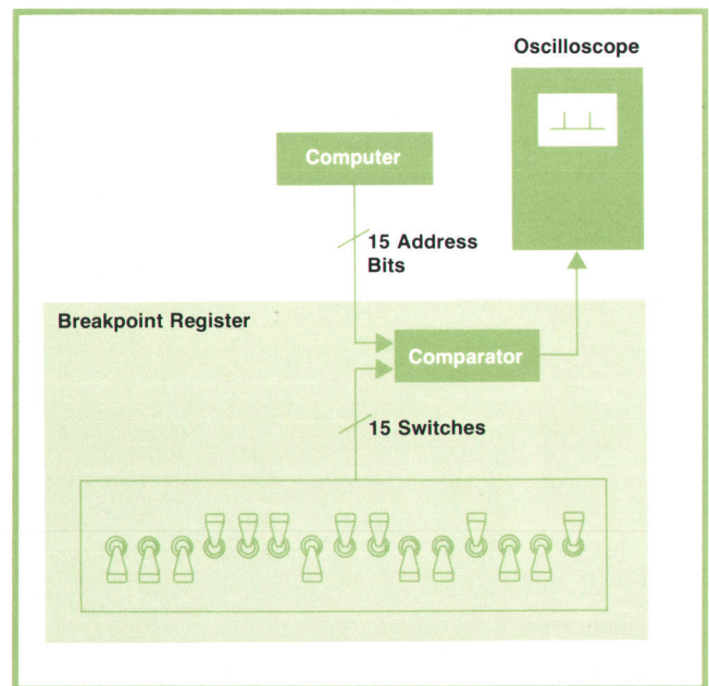
Fig. 2. A useful tool for timing analysis is a hardware breakpoint register, which emits a pulse whenever the computer program accesses the memory location set into the switch register. The comparator output may be displayed on an oscilloscope or be fed to a computer, even the one being measured.
